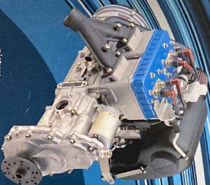
picture ROTAX® 582 UL DCDI with options
